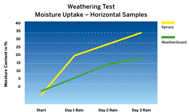
Figure 57. Water absorption of Spruce WeatherGuard and untreated spruce plywood measured by Metsä Wood.
