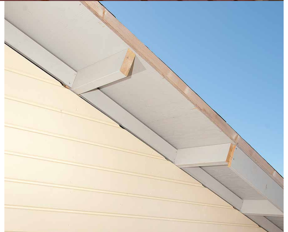
Figure 24. Cantilevers supporting eaves overhang
