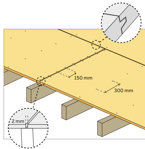
Figure 26. Metsä Wood Spruce (TG2) panel installation on rafters
