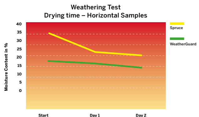
Figure 58. Drying time of Spruce WeatherGuard and untreated spruce plywood measured by Metsä Wood.
