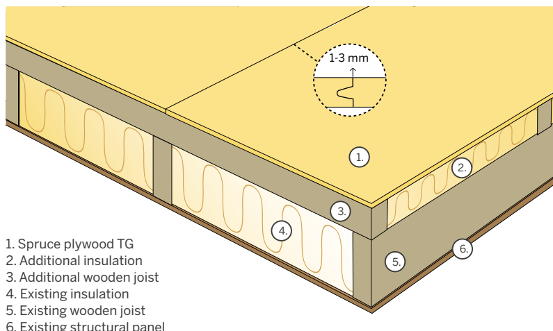
Figure 48. Additional insulation for base floor
