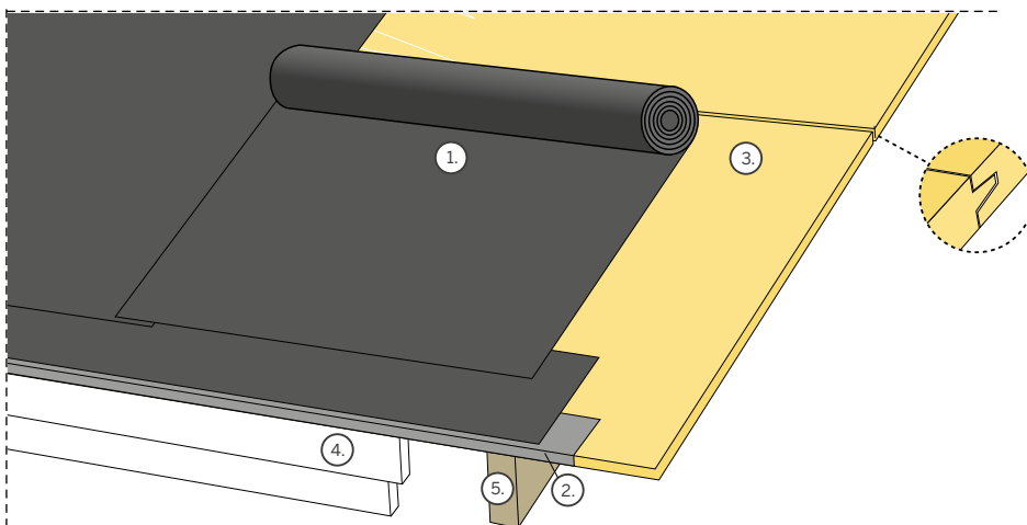
Figure 19. Roofing felt
