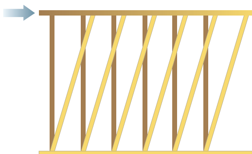
Figure 36. Laterally loaded wall structure without panel bracing
