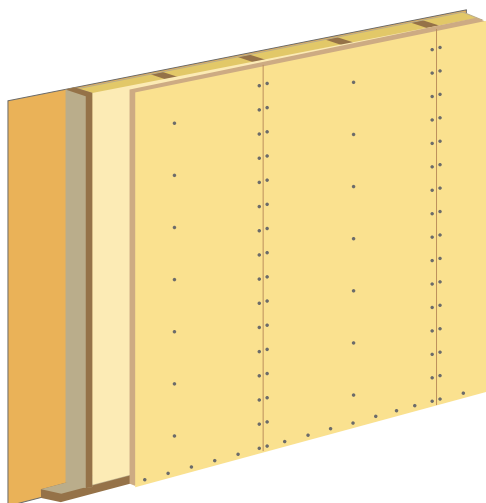
Figure 35. Panel bracing
