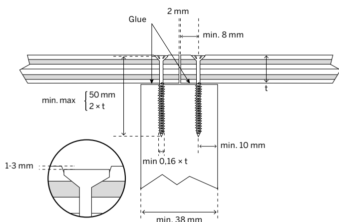
Figure 13. Fixing of square edge panels to wooden support
