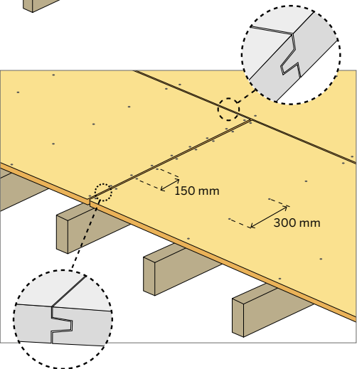
Figure 12. Metsä Wood Spruce (TG4) panel installation on floor joists
